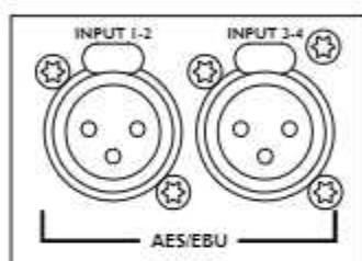
Figure 8.12: AES Inputs
