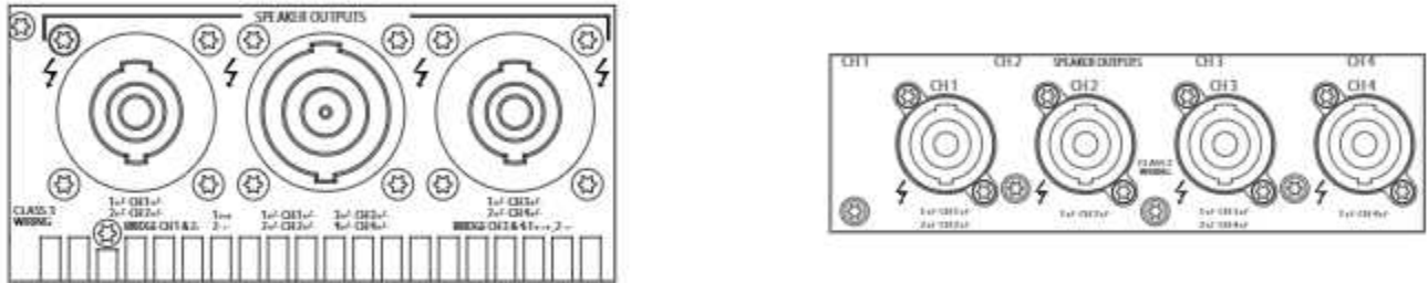
Figure 8.2: speakON Connections
