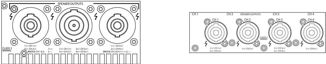
Figure 8.2: speakON Connections
