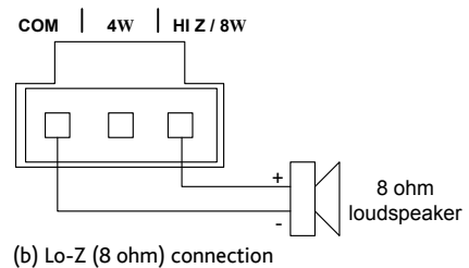
(b) Lo-Z (8 ohm) connection
