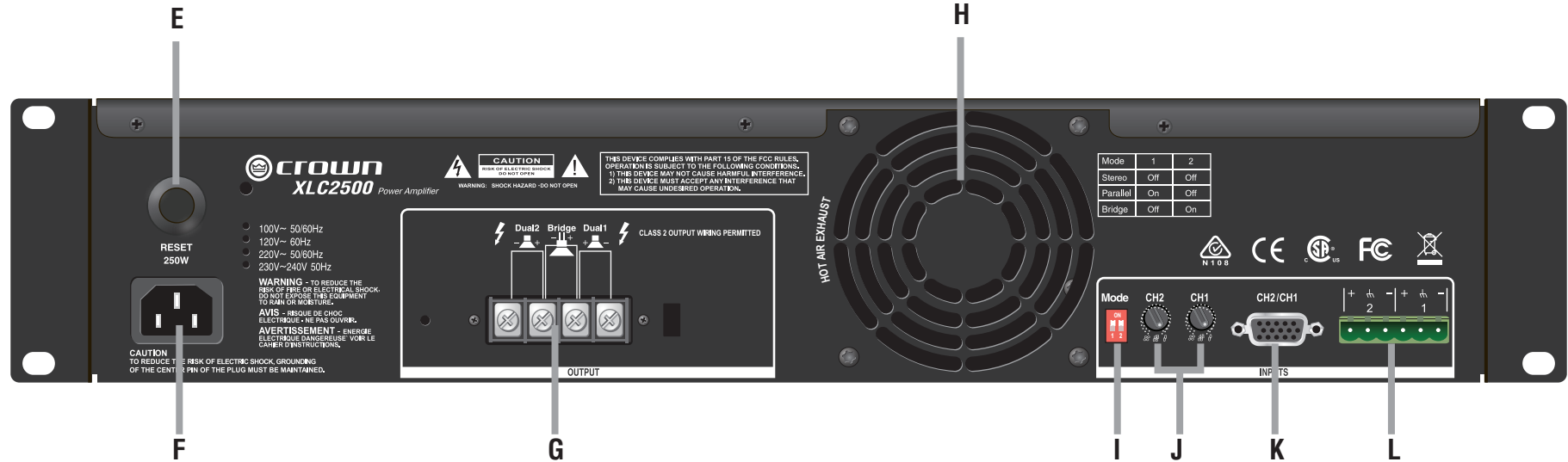
Figure 3.2 Rear Panel 图3.2 后面板
