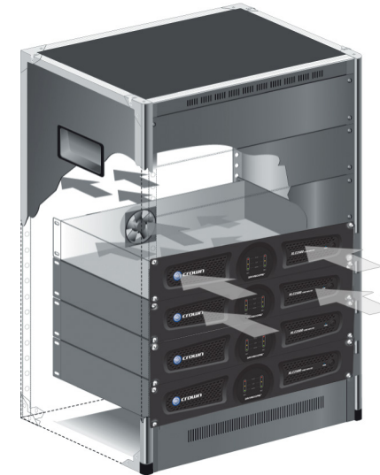
Figure 2.3 Airflow
