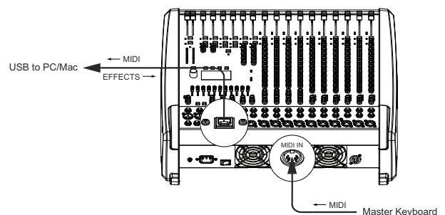
Illustration 4-6: Using the PC/Mac as MIDI tone generator (illustration shows PowerMate 1000-3)
