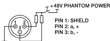
Illustration 2-10: Pin assignment of XLR microphone input
