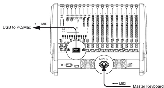
Illustration 4-5: Sending MIDI data from a Master Keyboard to a PC/Mac
