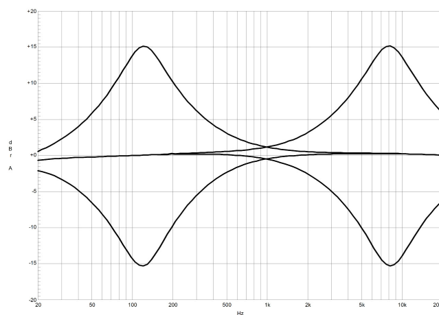
Illustration 2-8: MID filter
