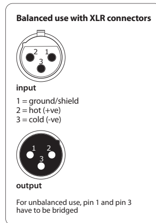
Fig. 4.2: XLR connections
