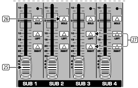
Fig. 2.9: Subgroups 1 - 4
