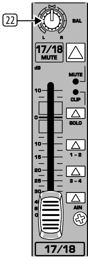
Fig. 2.7: Channel fader, balance control, mute switch, etc.
