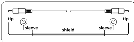
Fig. 5.3: RCA cable
