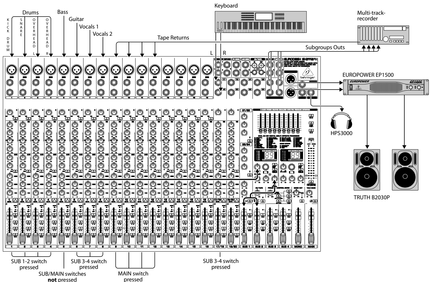
Fig. 4.1: Wiring the console for studio operation
