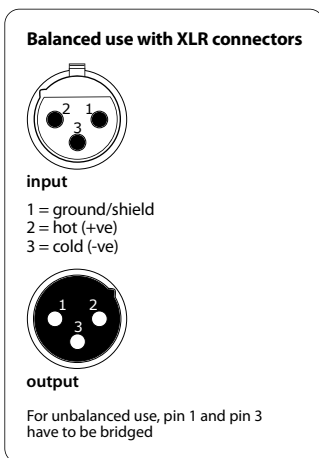
Fig. 5.4: XLR connectors
