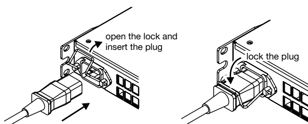
FIG. 4: Mains connector.
