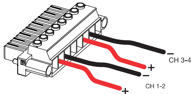
Phoenix PC 5/ 8-STF1-7,62 1777891
