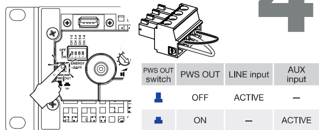
FIG. 3: Manual procedure to switch from LINE to AUX.
