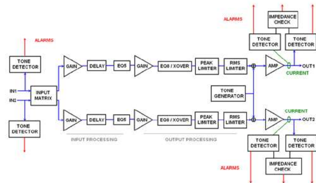
FIGURE 29: DSP processing blocks
