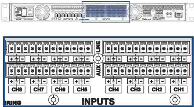
FIGURE 20: Rows of input connectors
