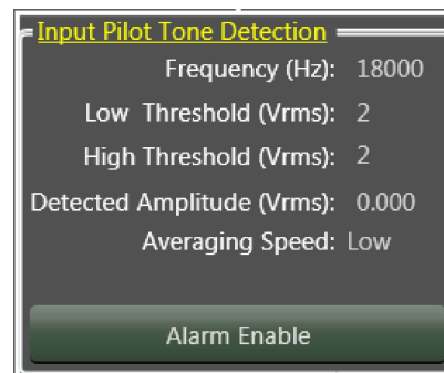
FIGURE 57: This control shows the threshold, the frequency and the measured amplitude of the tone.
