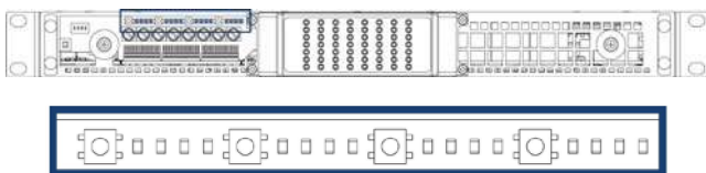
FIGURE 16: Front panel left hand side DSP LEDs
