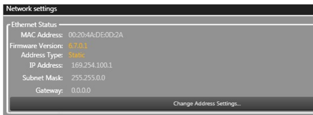
FIGURE 32: Select the static IP policy
