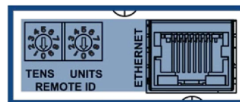
FIGURE 30: Rear Ethernet port and ID selection
