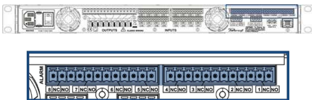
FIGURE 26: Back panel alarm output connectors
