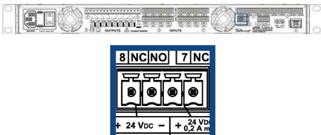
FIGURE 21: AUX SEL connector
