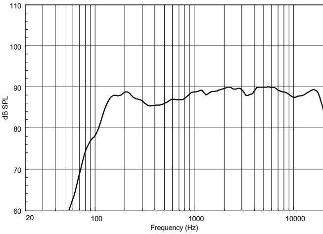
Response 1W/1m
