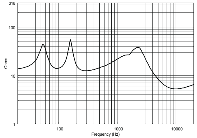
Impedance
