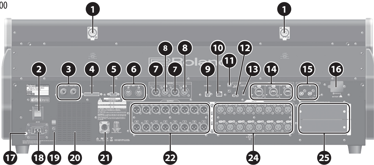
M-5000C
